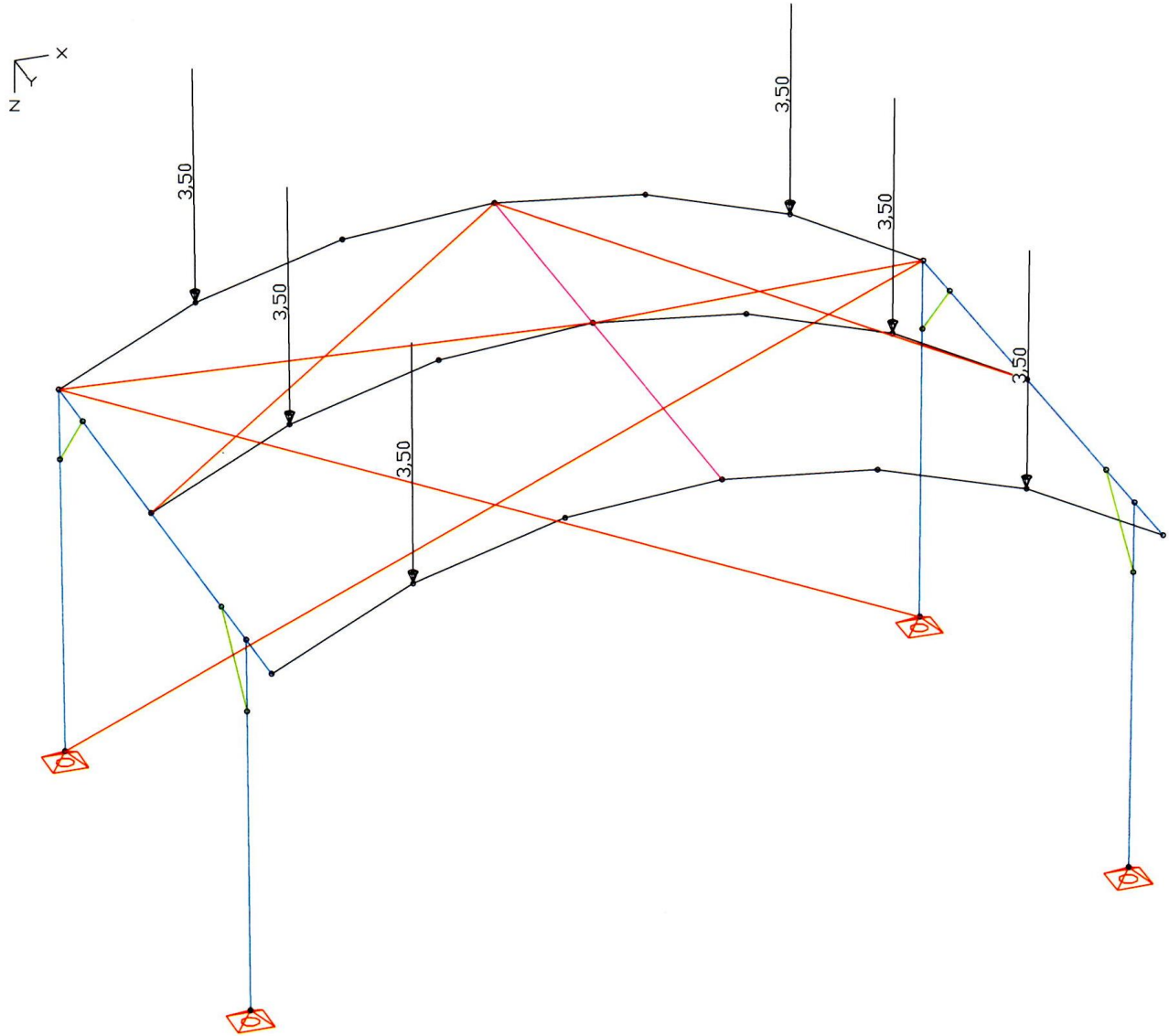
LF 4: Belastung, point load setup2
