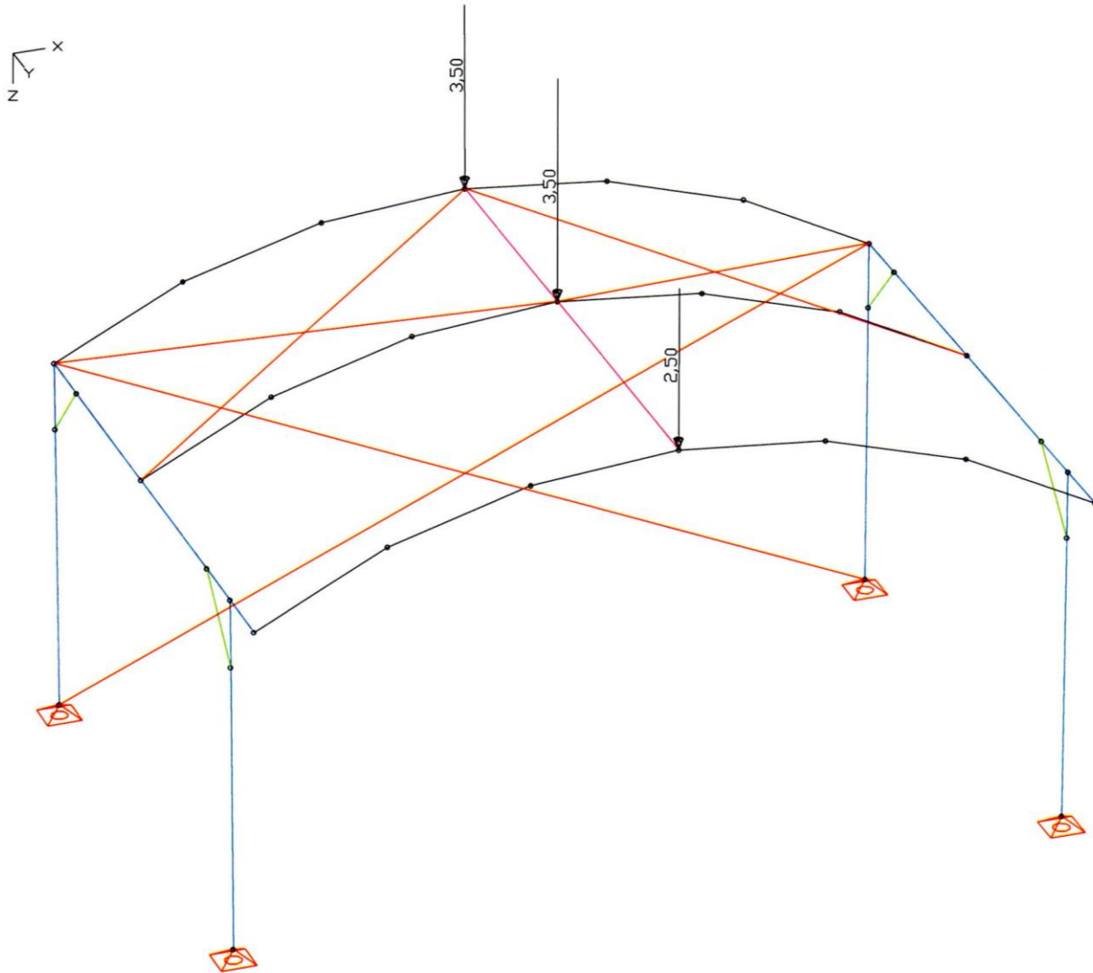
LF 3: Belastung, point load setup1
